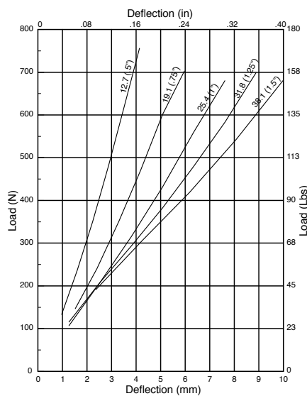
FIG. 5 P0500-XXXX-60A
