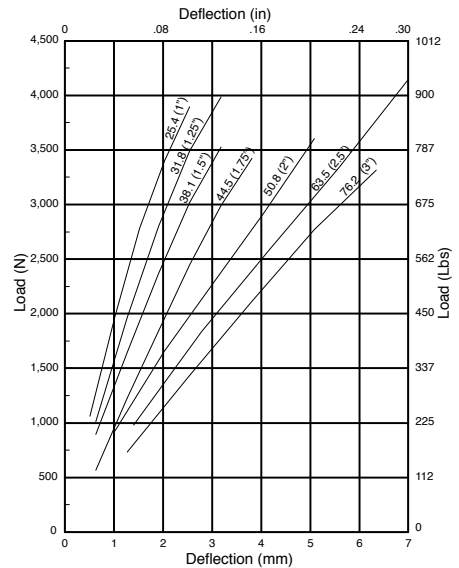
FIG. 27 P1000-XXXX-90A
