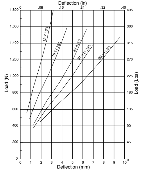
FIG. 21 P0312-XXXX-90A
