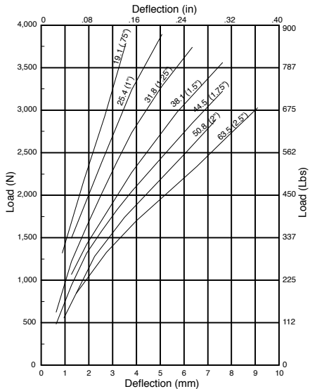
FIG. 25 P0750-XXXX-90A
