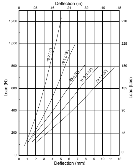
FIG. 6 P0625-XXXX-60A
