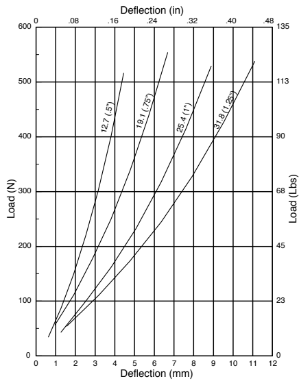
FIG. 1 P0188-XXXX-60A
