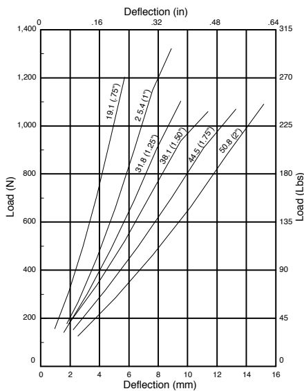
FIG. 7 P0750-XXXX-60A
